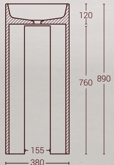
CROSS-SECTION VIEW
