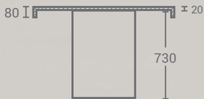
CROSS-SECTION VIEW
